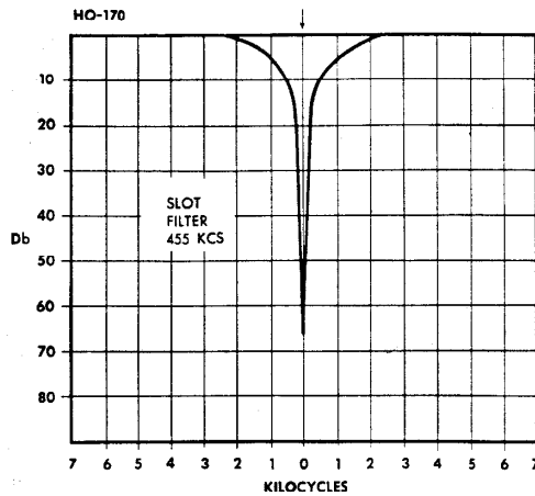
Figure 6. Slot Filter Response Curve
