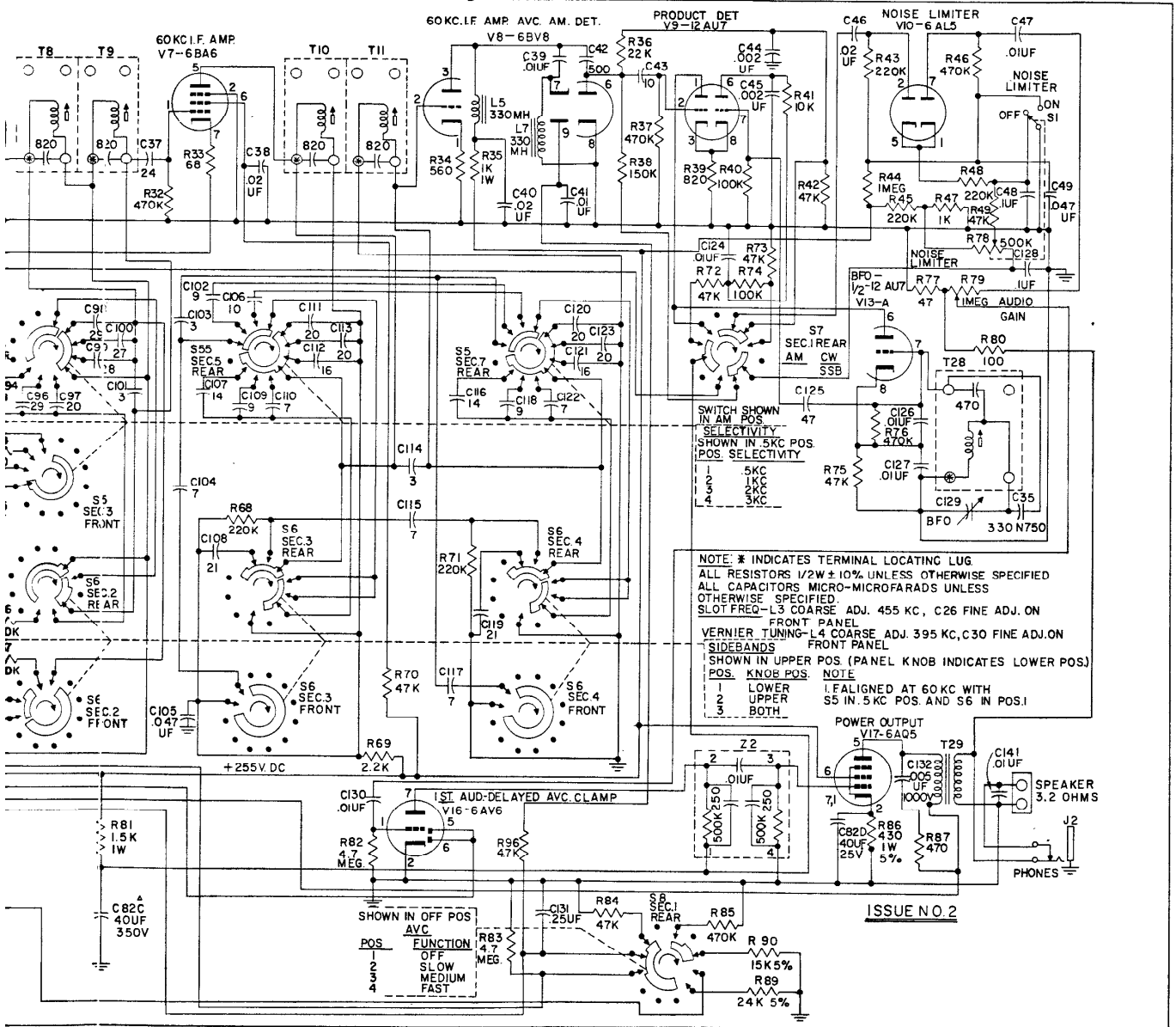
Figure 14. Hammarlund HQ-170 Communications Receiver, Schematic Diagram
