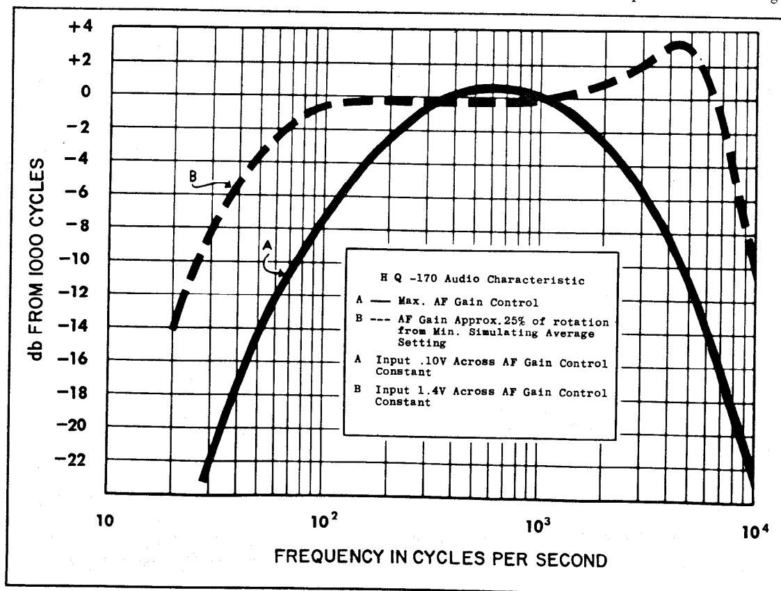
Figure 8. Auto-Response Curve
