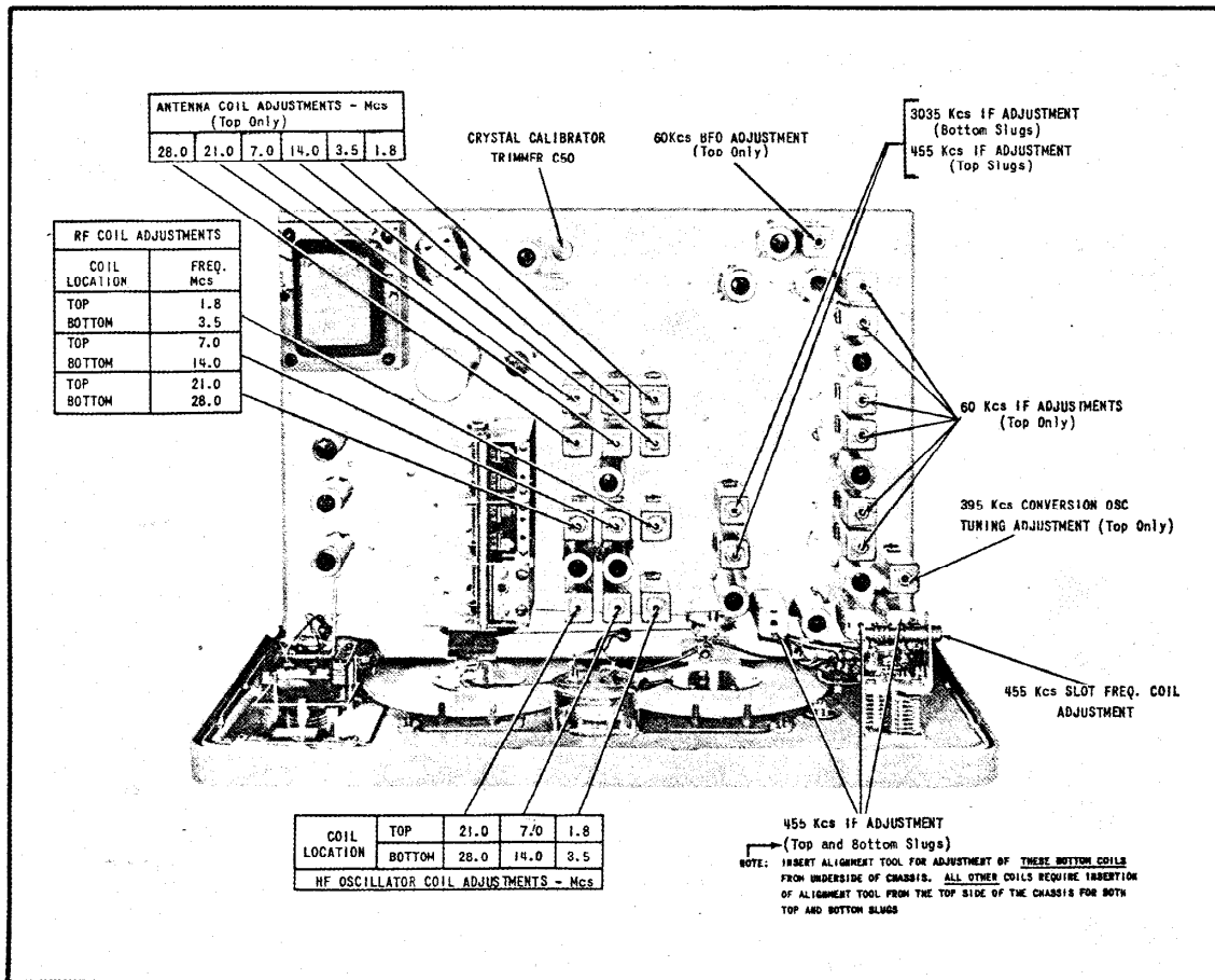
Figure 9. Top View of Chassis
