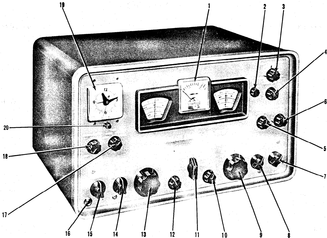
Figure 5. Location of Controls
