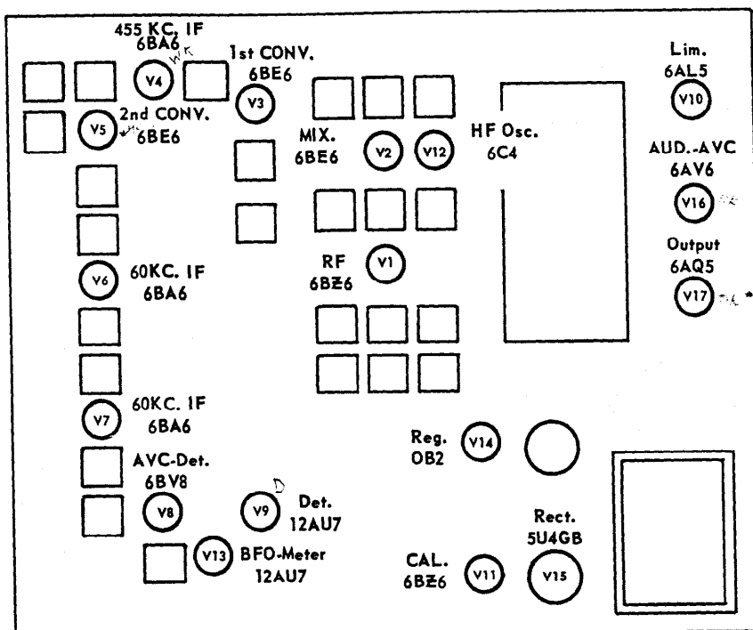
Figure 13. Tube Location Diagram
