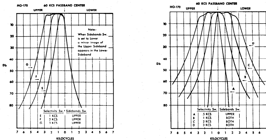
Figure 7. IF Passband Response Curves
