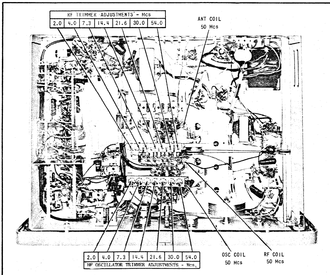
Figure 10. Bottom View of Chassis
